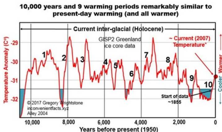
Figure 7.8 10,000 years of warming
