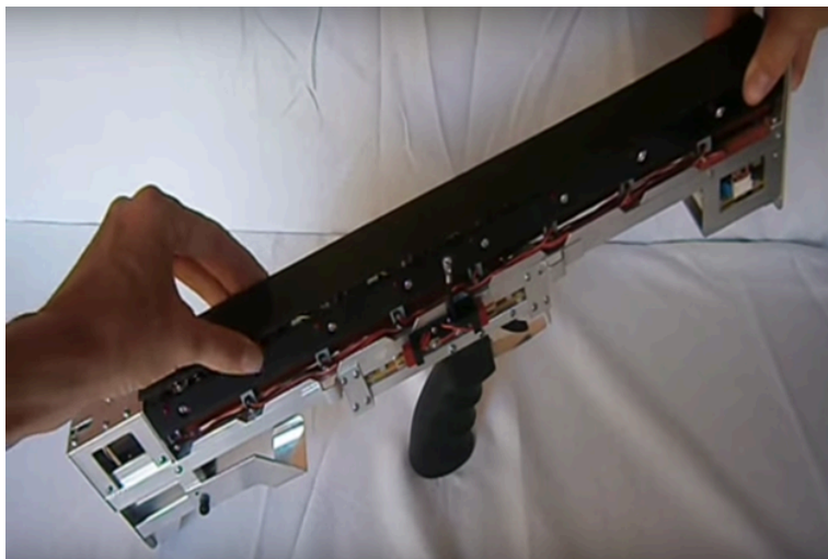
Figure 5.25 Coil gun
