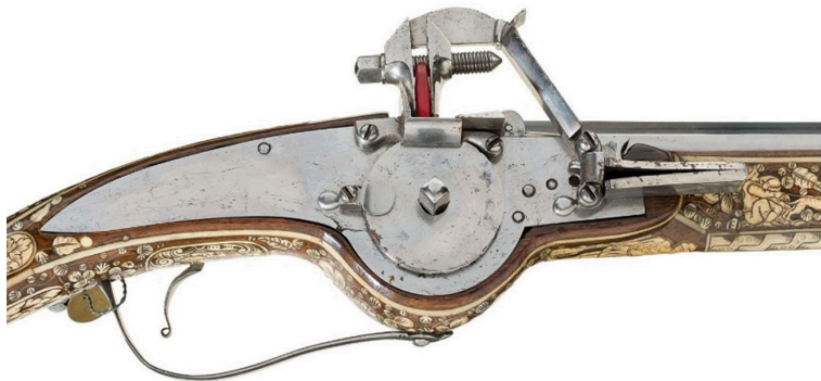
Figure 5.4 Wheel-Lock
