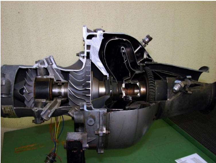
Figure 1.2 Cross section of a typical gas turbine engine. Courtesy of Tilyudai and reused under license CC BY-NC-SA 2.0. To view a copy of this license, visit https://creativecommons.org/licenses/by-nc-sa/2.0/ .
