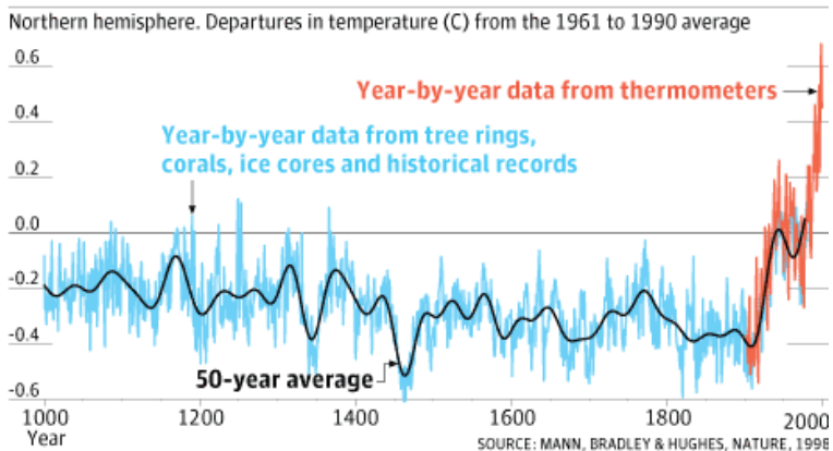
Figure 7.6 Mann-made Hockey Stick
