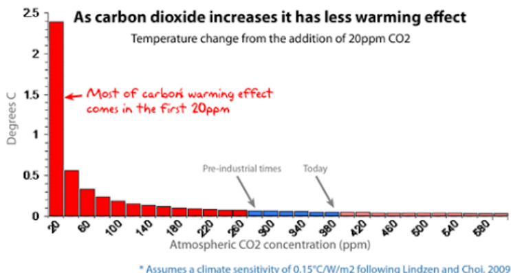
Figure 7.2 The diminishing influence of increasing Carbon Dioxide on temperature
